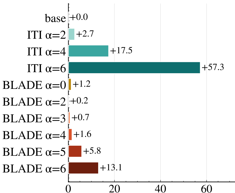
(a) capability cost \Delta perplexity (%) ↓
