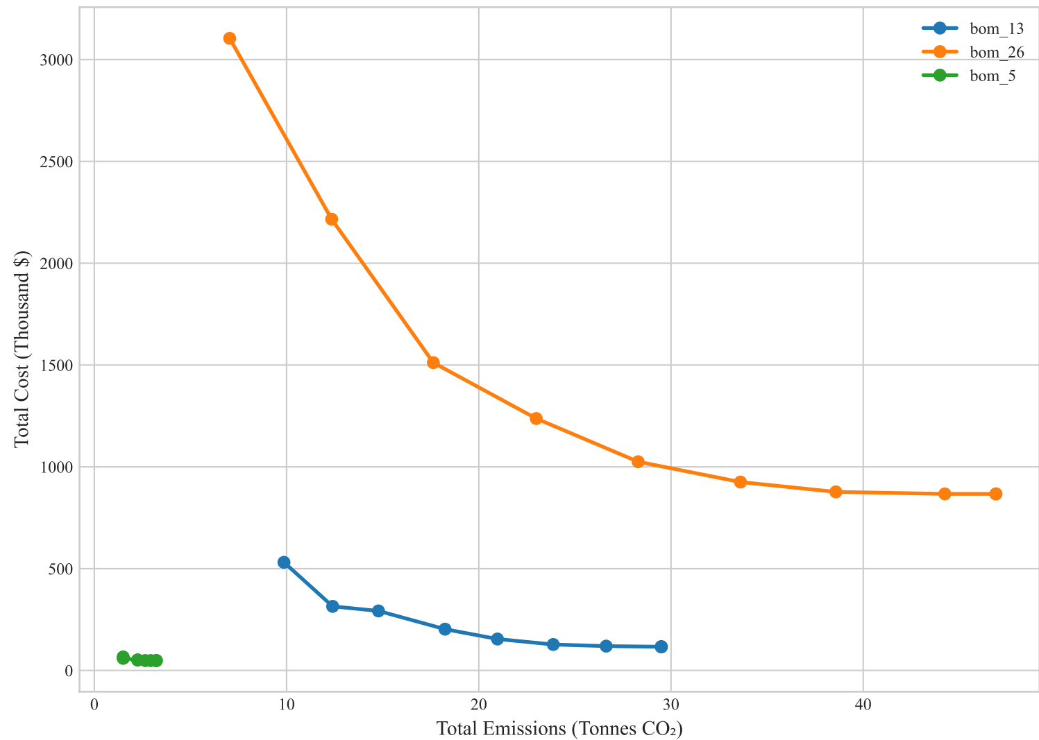
Cost-Emissions Pareto Front
