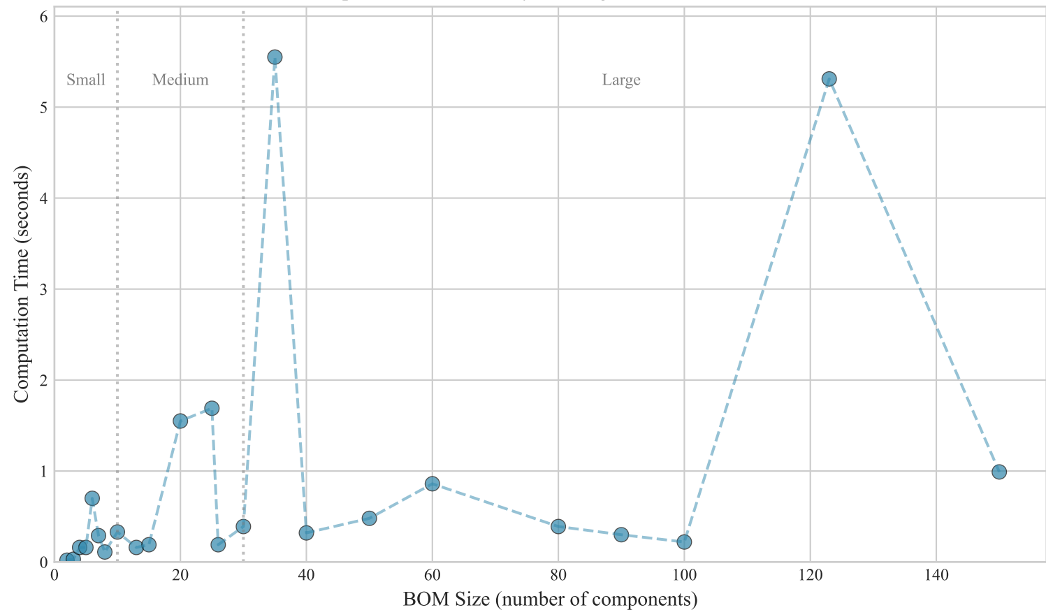
Computational Scalability of Integrated DDMRP Model
