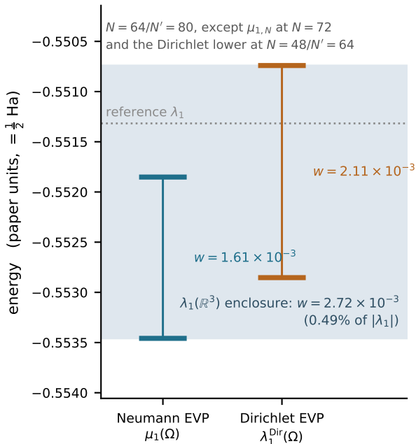
(a) L = 10 : every endpoint certified
