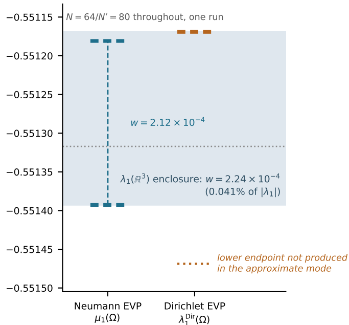
(b) L = 14 : approximate mode, not bounds
