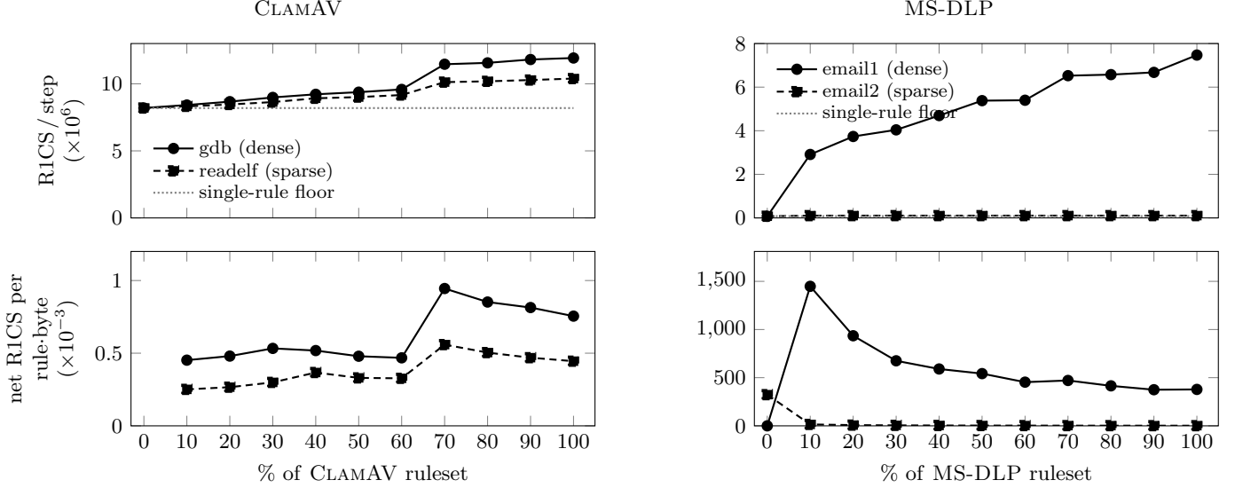
Figure 1: Ruleset-size scalability (input fixed), per folding step, on CLAMAV (left) and MS-DLP (right). Top : absolute circuit size with the single-rule framework floor (dotted; 8.19M R1CS for CLAMAV, 0.08M for MS-DLP); growing the ruleset to the full 38,875 (CLAMAV) / 9,861 (MS-DLP) rules grows the circuit far slower than the rule count. Bottom : net circuit cost per rule per input byte —cumulative R1CS above the floor divided by cumulative rule count times per-step input length—falling from 0.94 \times 10^{-3} to 0.76 \times 10^{-3} (gdb) and 0.56 \times 10^{-3} to 0.44 \times 10^{-3} (readelf) R1CS per rule-byte (CLAMAV) and 1448.30 \times 10^{-3} to 378.03 \times 10^{-3} (email1) and 323.59 \times 10^{-3} to 1.53 \times 10^{-3} (email2) R1CS per rule-byte (MS-DLP) at the full set. For the same MS-DLP ruleset, ZOMBIE emits 77,463,552 R1CS in total; dividing by the 2000-byte input and the same 9,861 rules gives \sim 3.93 R1CS per rule-byte, the same normalization applied to BORA.
