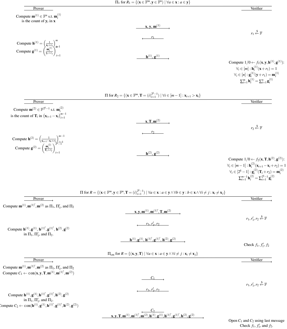
Figure 8: Protocols for Example 3
