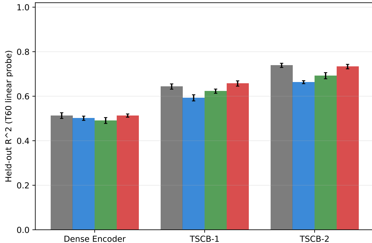
mean-pooled probe
