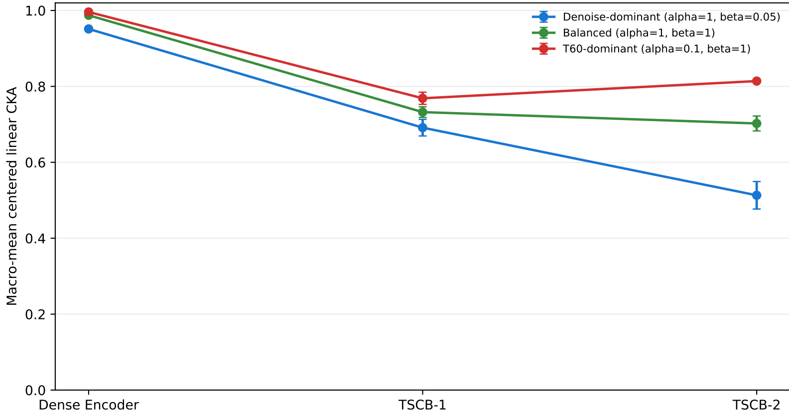
Representation similarity across weighting configurations
