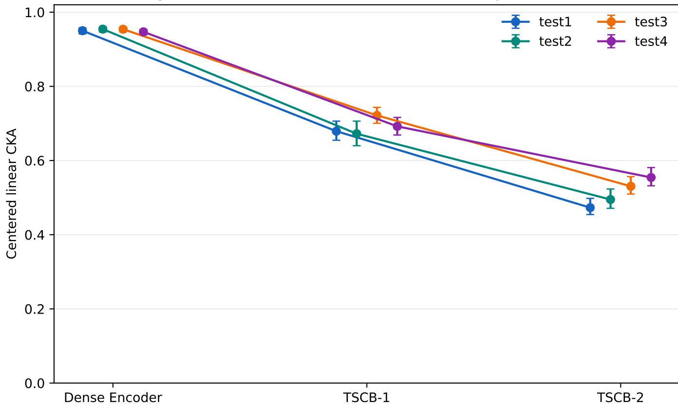
Single-task vs. denoise-dominant multi-task representations
