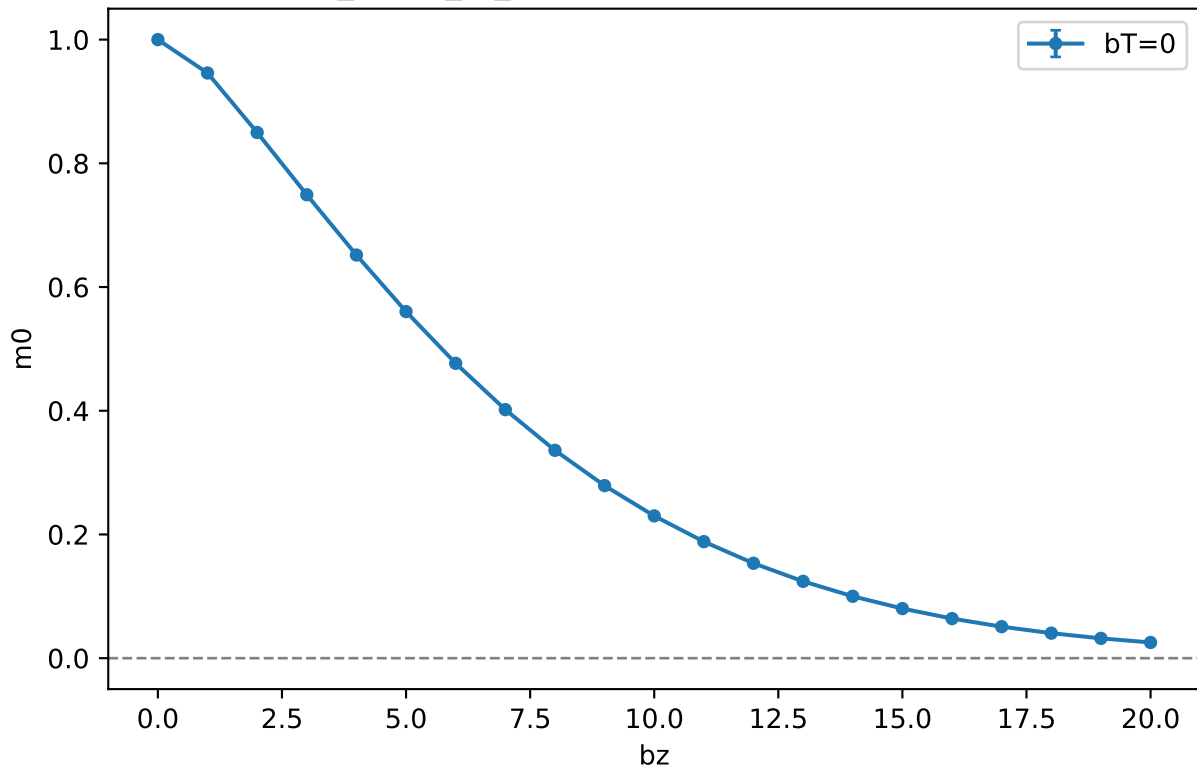
l64c64a076_m140_fit_pz1 T5 eta0 mode3 real 2state m0 vs bz
