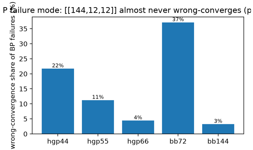
Figure 3: Wrong-convergence share of BP failures at p = 0.1 across the sampled codes (surface patches: avoidable failures; bicycle codes: all failures).
