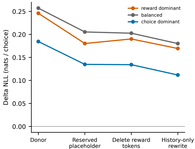
LLaMA SFT (one seed)
