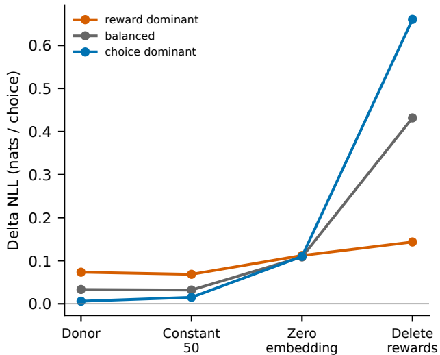
Transformer (one seed)
