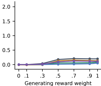
Previous reward only
