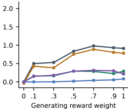
Suffix rewards only
