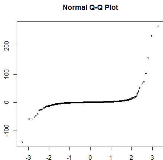
QQ-Plot 1
