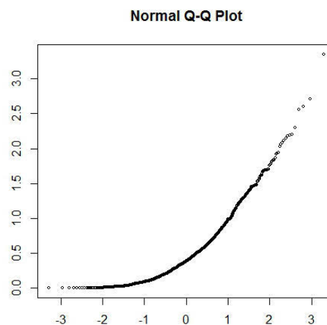
QQ-Plot 4
