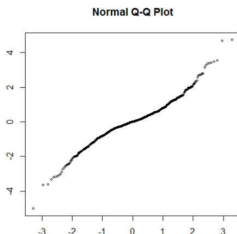
QQ-Plot 5
