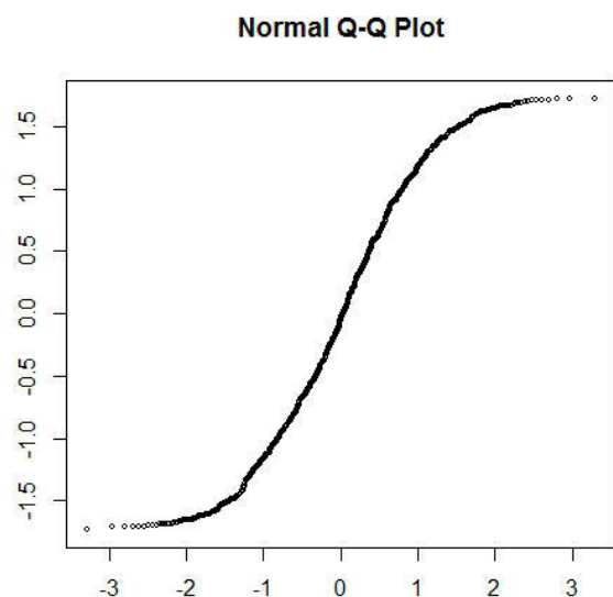
QQ-Plot 2
