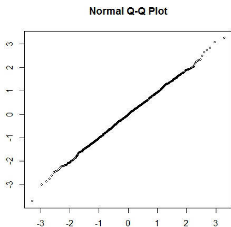
QQ-Plot 3
