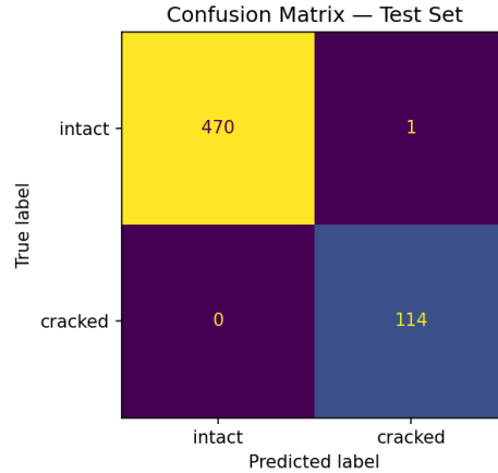
Figure 11: EfficientNet-B4 confusion matrix on the HistoricalCrack18-19 test set (585 images). Zero false negatives: every cracked image is correctly flagged. One false positive: one intact image predicted as cracked.
