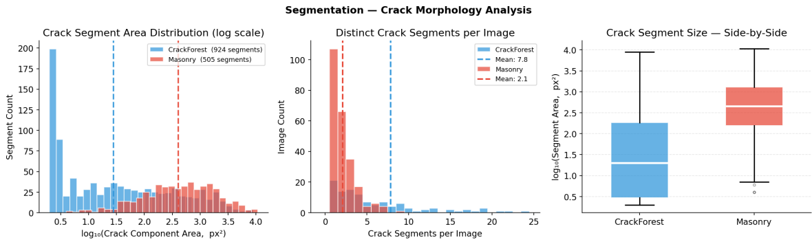
Figure 8: Crack morphology analysis via connected-component labelling. Left: log-scale distribution of crack segment area ( \text{px}^2 ) per dataset; dashed lines indicate class means. Centre: number of distinct crack segments per image. Right: box-plot comparison of log segment area. CrackForest has more, smaller segments; Masonry has fewer, larger ones.
