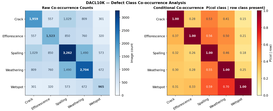
Figure 5: DACL10k defect class co-occurrence matrix. Left: raw image counts per class pair (diagonal = total images containing that class). Right: conditional probability P(\text{col class} | \text{row class present}) , row-normalised. High off-diagonal values indicate classes that reliably co-occur, motivating joint multi-label detection.
