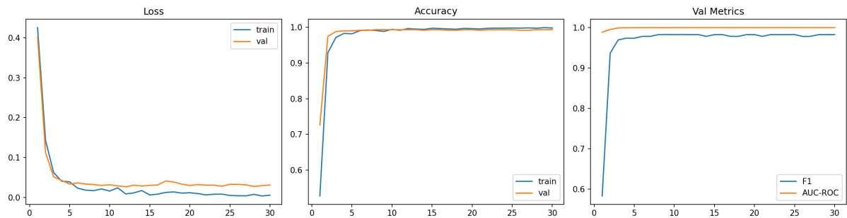
Figure 10: EfficientNet-B4 training curves over 30 epochs. Left: train/val loss converges rapidly by epoch 5 with no divergence. Centre: train/val accuracy both plateau above 99%. Right: validation F1 and AUC-ROC; AUC-ROC reaches 1.00 by epoch 3, confirming perfect class separation at any threshold.
