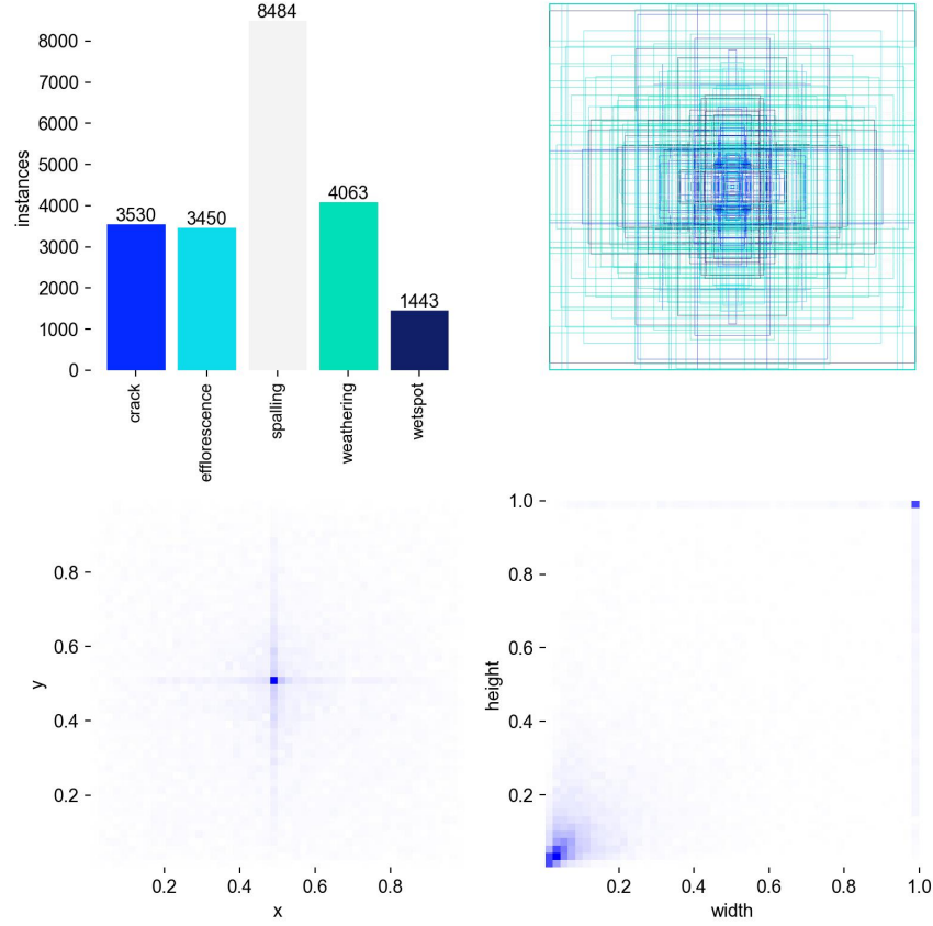
Figure 14: DACL10k v2 training split annotation statistics. Top-left: per-class instance counts (spalling dominates at 8,484 boxes; wetspot is least represented at 1,443). Top-right: bounding box spatial distribution (most boxes cluster centrally). Bottom: box centre and size distributions, showing the majority of damage annotations are small-to-medium sized and spatially centred, consistent with close-range bridge inspection photography.
