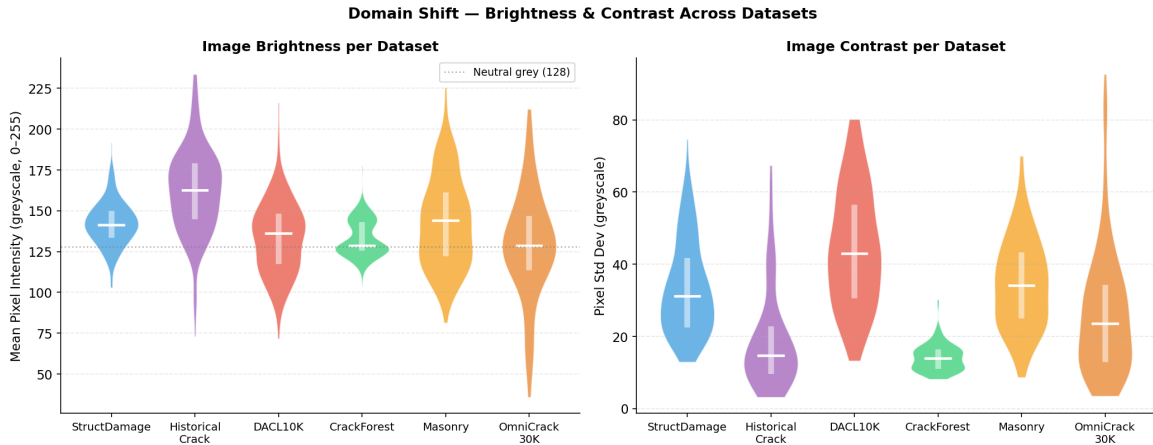
Figure 4: Domain shift quantified via brightness (mean greyscale intensity) and contrast (pixel std dev) across all six datasets. Each violin shows the full distribution over 120 sampled images; the white bar spans the interquartile range. Datasets below the neutral grey line (128) will produce systematically different activations in an ImageNet-pretrained backbone, motivating colour jitter augmentation.
