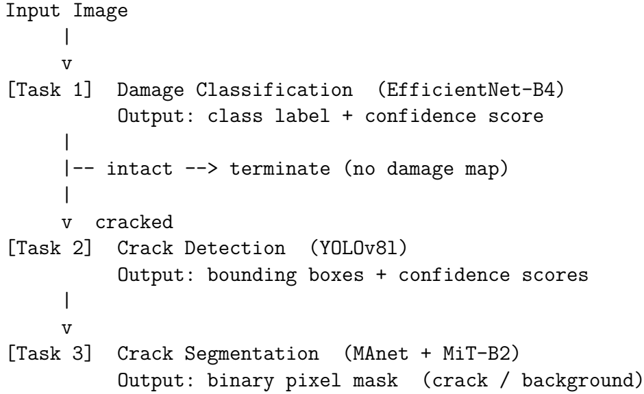
Figure 9: Three-stage inference pipeline. Task 1 acts as a gate: intact images are rejected before the computationally expensive detection and segmentation steps, eliminating false-positive detections on undamaged surfaces.
