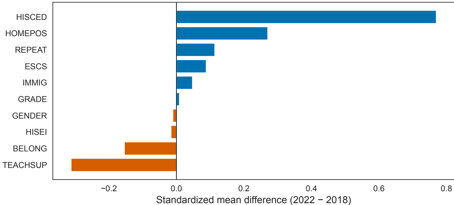
Feature Drift: 2022 vs 2018 (Cohen's d)
