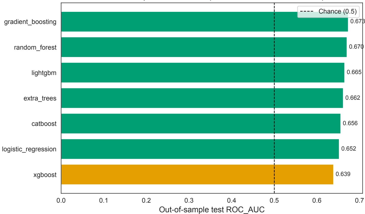
Out-of-Sample Performance (train 2009–2018 → test 2022)
