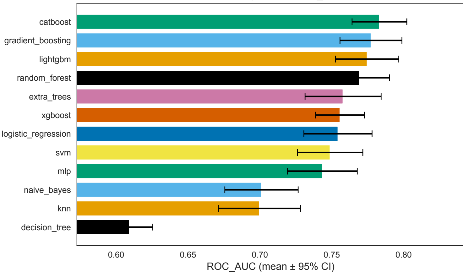
Model Comparison: ROC_AUC
