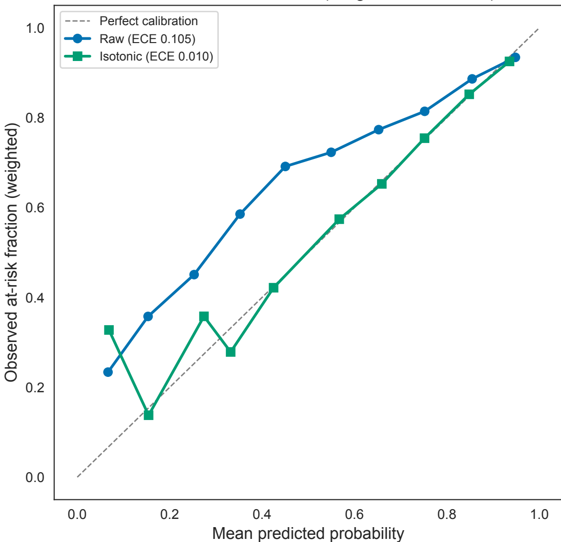
Calibration: Albania 2022 (weighted, out-of-fold)
