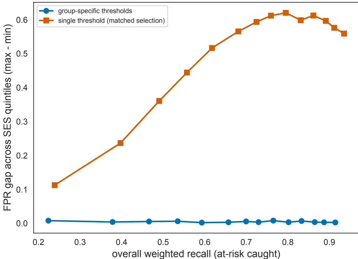
Fairness-utility trade-off: mitigating SES over-flagging (2022)
