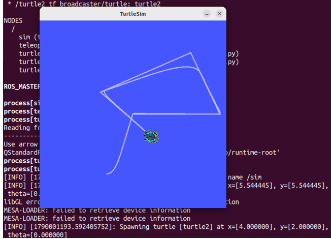
Fig. 21. The standard turtle TF demonstration with the simulator and TF nodes running.
