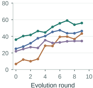
BFCL multi-turn
