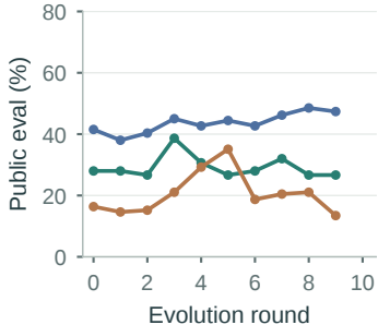
\tau^2 -Bench
