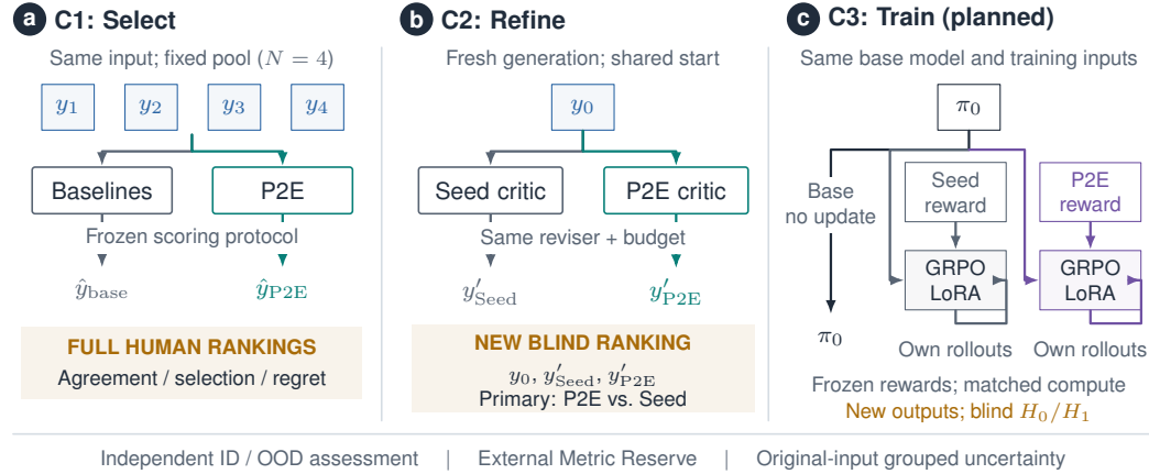
Figure 5: Three controlled uses of the evolved evaluator. Panel (a), C1, holds the candidate pool fixed and compares ranking and selection. Panel (b), C2, branches from a freshly generated shared y_0 and changes only the critic. Panel (c), C3, contrasts an unchanged Base policy with two policies trained under frozen rewards. The trained policies use matched inputs and compute but generate their own rollouts. Final judgments are blinded and external metrics are reserved from evolution. C3 is a planned training study, not an executed experiment.
