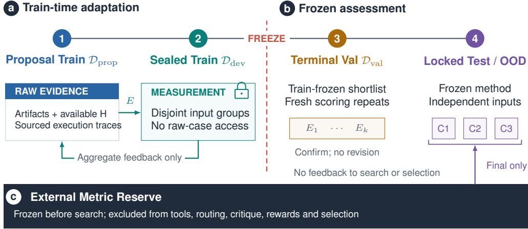
Figure 7: Data and metric boundaries. Panel (a) exposes raw proposal-Train evidence but returns only aggregate measurements from a disjoint sealed Train cohort. Panel (b) assesses a frozen shortlist on Val and the frozen method on locked Test/OOD. Panel (c) reserves metrics for independent final assessment. The reserve cannot be reintroduced through tools, critique, reward, aliases, or checkpoint selection. All partitions preserve original-input/source groups.
