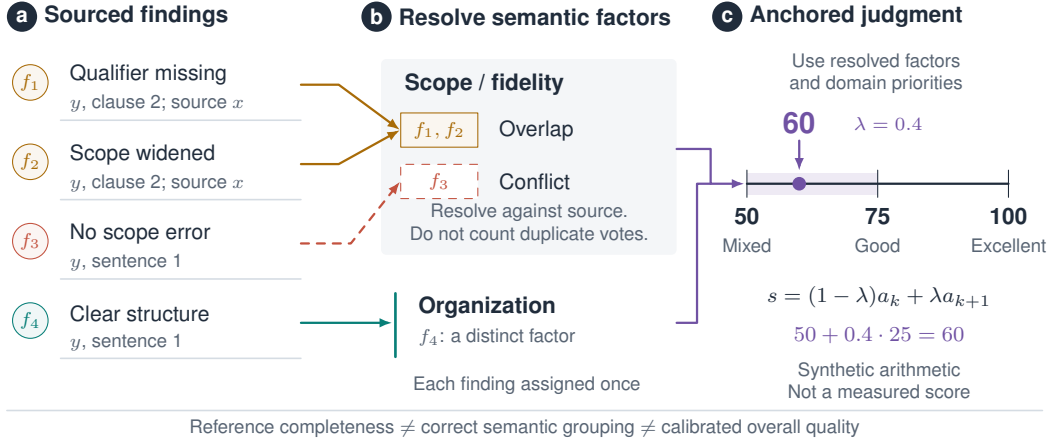
Figure 8: Optional semantic synthesis. Panel (a) supplies sourced findings; (b) groups overlapping and conflicting statements into factors; (c) locates overall quality between prespecified anchors. Every finding reference is assigned once, but bookkeeping alone cannot validate the grouping or the quality judgment. The anchor values and interpolation are a synthetic arithmetic example, not an evaluator result or a universal scale for all domains.
