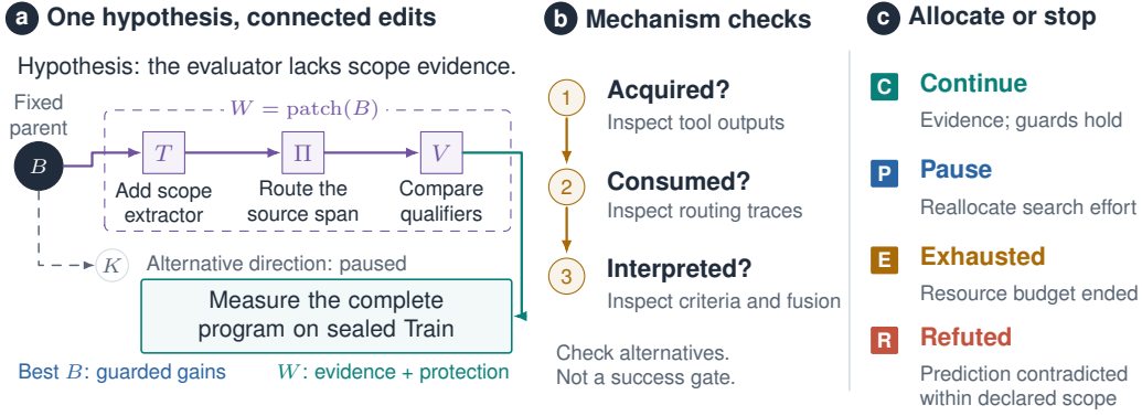
Figure 4: A direction is a hypothesis, not an edit. (a) Connected tool, routing, and interpretation changes share a fixed parent. Best and working programs remain distinct; promotion and continuation both require complete measurement. (b) Check evidence acquisition, consumption, and interpretation. (c) Distinguish continuation, pause, exhaustion, and scoped refutation. The revision branches are schematic, not an observed optimization trajectory.
