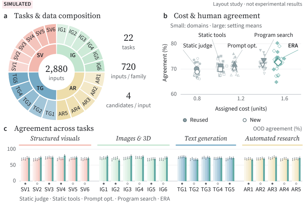
Figure 4: Simulated task coverage and evaluator comparisons; not experimental results. Panel (a) summarizes 22 tasks and 2,880 input groups, balanced to 720 per family with four candidates per input. A fixed hash selects this subset without reading outcomes; the appendix reports the full synthetic cohorts. Sector angles encode input counts; task codes follow Table 3. Panel (b) plots assigned cost units, not measured runtime, against OOD agreement with synthetic human rankings. Small marks denote 110 domain–method combinations; large marks equally average 11 domains per feedback setting. Shapes identify methods, and filled/open marks denote illustrative reused/new preferences, not label reliability. Panel (c) reports agreement from pointwise scores and 95% input-group bootstrap intervals on a common 0–100% scale. Baseline bars follow the displayed order in each family’s hue; ERA is lake green. Cost includes all selected inputs; agreement uses method-complete inputs. Marginal intervals do not establish paired differences.
