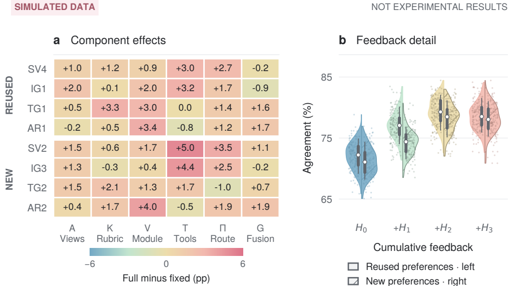
Figure 9: Simulated ablations; not experimental results. Panel (a) gives mean full-minus-fixed agreement (percentage points) for (A, K, V, T, \Pi, G) across eight diagnostic domains, with cream at zero. Panel (b) colors cumulative H_0-H_3 levels. Left/right halves denote reused/new preferences; right halves are hatched. Dots are synthetic groups, white markers medians, thick segments quartiles, and thin segments the 10th–90th percentiles. Domain codes follow Table 13. Conditional contrasts are not additive contributions or evidence of component benefits.
