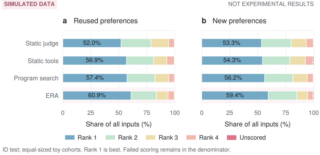
Figure 8: Simulated C1 selection; not experimental results. Panels (a) and (b) show horizontal rank profiles for four evaluator fixtures in the two construction settings, using ID inputs. Rank 1 is best. Labels give its share of all input groups, including unscored groups in the denominator. Colors encode ranks, not methods. Equal cohort sizes permit pooling within a setting; actual domain-level results must also be reported.
