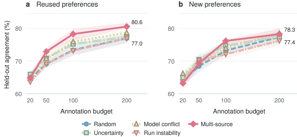
Figure 6: Simulated acquisition curves; not experimental results. Panels (a) and (b) compare five policies under reused and newly collected preferences. Lines average 12 toy runs; bands mark each policy’s 10th–90th percentiles, not confidence intervals. Budgets count original-input annotation units, including a shared 10-unit random anchor.
