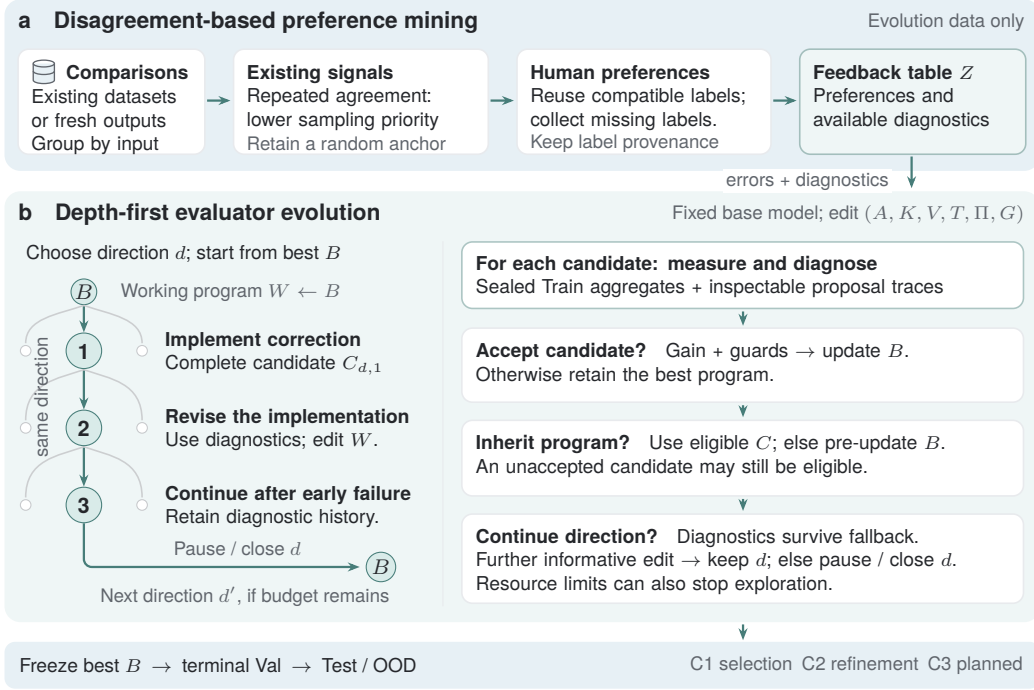
Figure 2: IterEval: from human preferences to an improved evaluation procedure. Panel (a) mines existing datasets or new outputs, reusing compatible preferences or collecting missing ones. Panel (b) shows successive revisions within a direction, with alternatives deferred until it pauses or closes. The green spine denotes editing opportunities, not automatic inheritance. Acceptance, inheritance, and continuation are separate decisions; fallback uses the pre-update best program and retains diagnostics. Terminal validation does not trigger edits or reranking. This is a method specification, not a result.
