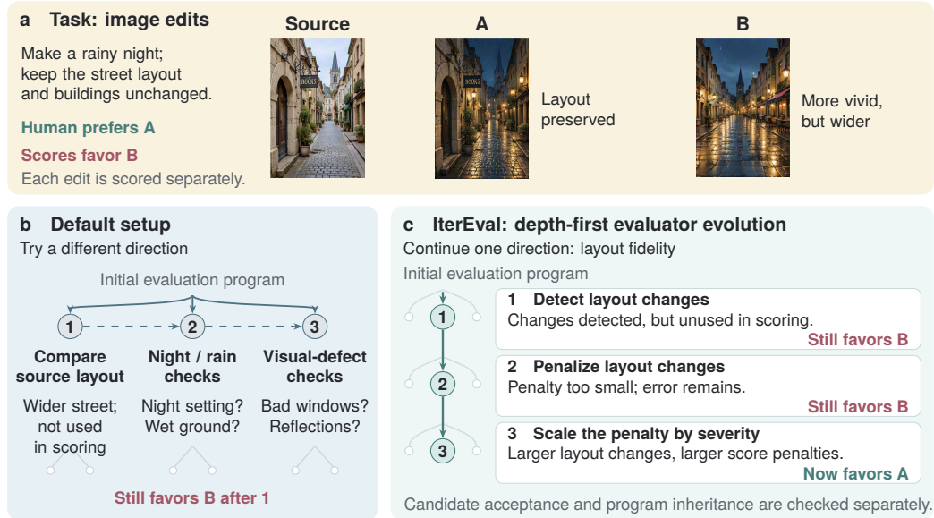
Figure 1: Dive deeper, branch later. Panel (a) contrasts layout fidelity with visual richness. Panel (b) branches across plausible corrections; dashed arrows show attempt order. Panel (c) develops one correction through detection, scoring, and severity weighting. Nodes denote complete evaluation programs; hollow nodes are unexplored alternatives. The corrected ordering is local to this example, not candidate acceptance or generalization. Images, preferences, and paths are constructed illustrations, not experimental evidence.
