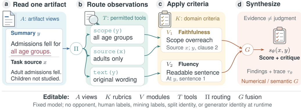
Figure 4: The six-component evaluation program. (a) Read one candidate and permitted task evidence. (b) Route tool observations. (c) Apply dimensional criteria. (d) Fuse sourced findings into a score and critique. The lower rail identifies the editable components. Human feedback supervises evolution, never the deployed scorer. Evidence and judgment remain separate; the summary and findings are a constructed example.
