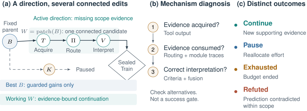
Figure 4: A direction is a hypothesis, not an individual edit. Panel (a) illustrates a fixed-parent sequence of tool, routing, and interpretation changes, alongside separate best-program and working-program states. Panel (b) asks whether evidence was obtained, consumed, and interpreted before drawing a direction-level conclusion. Panel (c) distinguishes continuation, pause, resource exhaustion, and scoped refutation. This is a schematic search tree, not an observed optimization trajectory.
