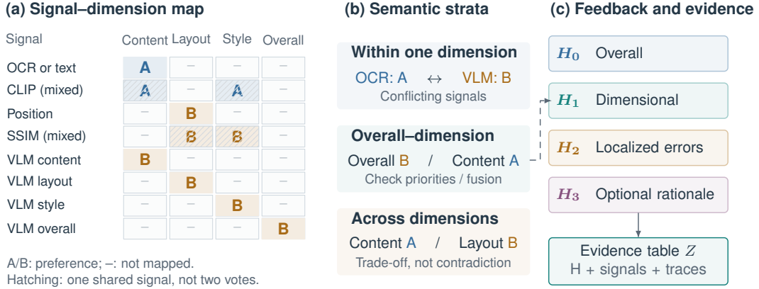
Figure 2: From evaluator signals to informative feedback. Panel (a) is a synthetic webpage example of the many-to-many signal-dimension mapping; letters indicate candidate preference, not scores. Hatched cells share one mixed signal. Panel (b) distinguishes within-dimension contradiction, overall-dimension disagreement, and a trade-off between different dimensions. Panel (c) connects these strata to H_0 – H_3 and the adaptation evidence table Z . The matrix is illustrative and does not report measured scorer behavior.
