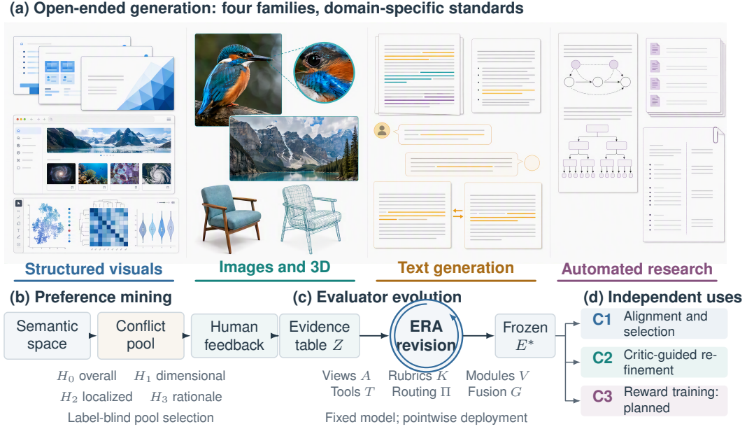
Figure 1: P2E connects an evaluation ecosystem to feedback acquisition, evaluator evolution, and independent downstream assessment. Panel (a) illustrates the four domain families; each domain retains its own evaluation standard. Panel (b) maps evidence, mines disagreements, and forms structured human feedback. Panel (c) uses ERA to revise a six-component program. Panel (d) separates alignment and selection (C1), refinement (C2), and planned reward training (C3). The GPT Image 2 artifact vignettes are synthetic illustrations, not experimental cases; arrows specify information flow, not measured improvements.
