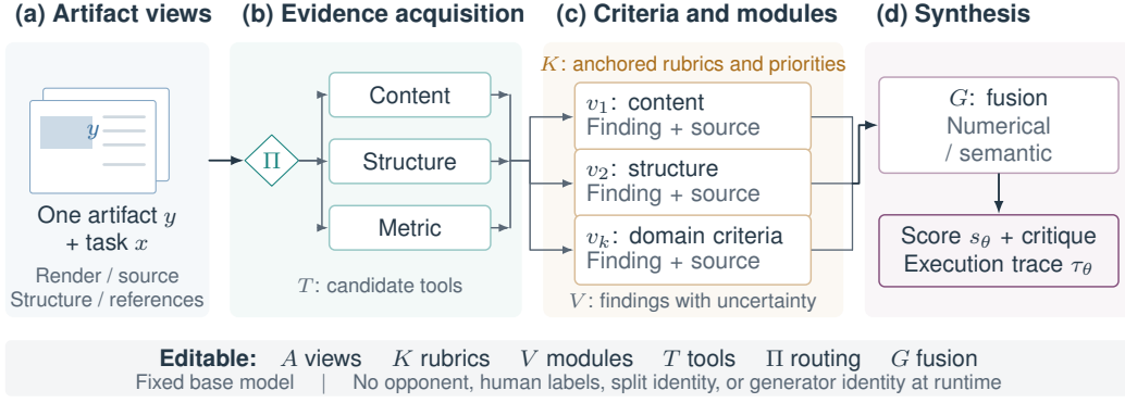
Figure 3: The six-component evaluation program. Panel (a) adapts one candidate and permitted task evidence; (b) routes observations from an executable tool library; (c) applies dimension-specific criteria through evaluator modules; and (d) fuses sourced findings into a score and critique. The lower rail identifies the editable components. Human feedback supervises the outer evolution process, never the deployed scoring path. Evidence and judgment are separate objects.
