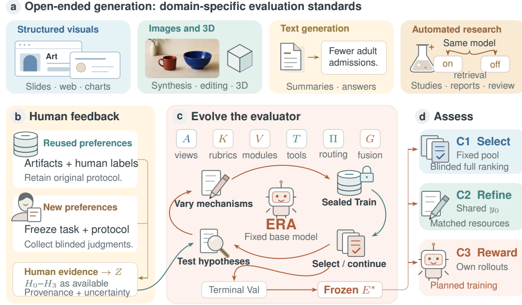
Figure 1: P2E evolves evaluation systems using human feedback. (a) Four artifact families retain distinct evaluation standards. (b) Reused and newly collected preferences enter a common evidence interface; their provenance and annotation quality remain separate. (c) ERA evolves a six-component program with a fixed base model. (d) C1 selection, C2 refinement, and planned C3 reward training. Artifacts and feedback are constructed illustrations; the photograph is generated with GPT Image 2. Arrows denote information flow, not measured improvements.
