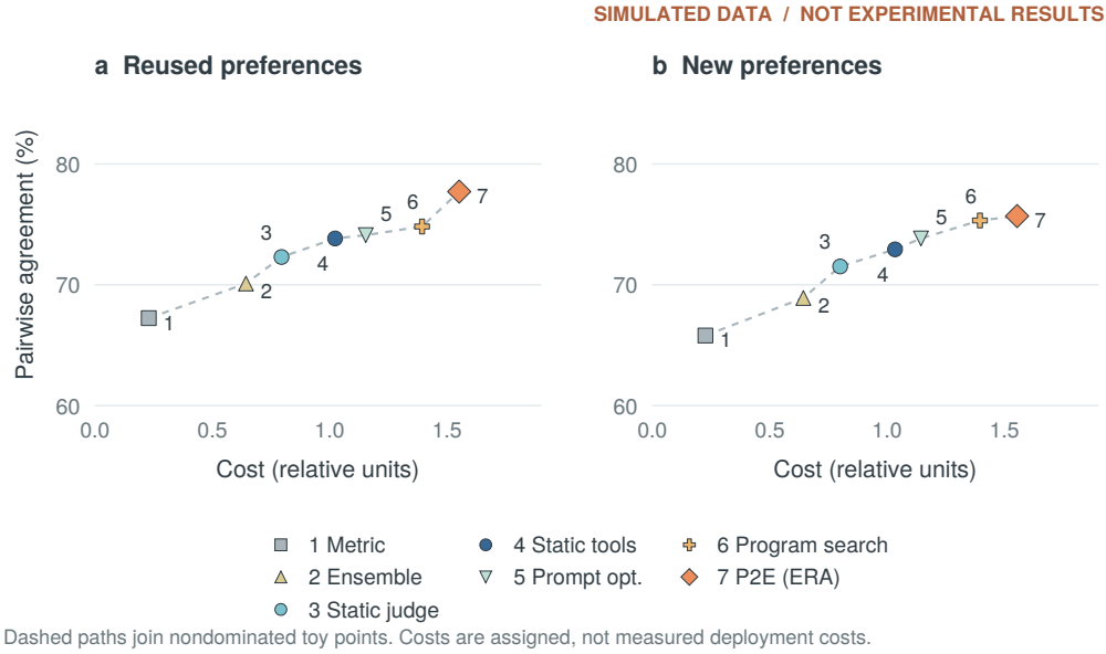
Figure 9: Simulated quality–cost trade-offs; not measured costs. Panels (a) and (b) give equal-weight means across four ID cohorts per setting. Markers identify evaluator fixtures and dashed paths join their nondominated points. Cost units are assigned to the toy generator, not timed API calls or measured compute. The plot does not establish an efficiency frontier for ERA.
