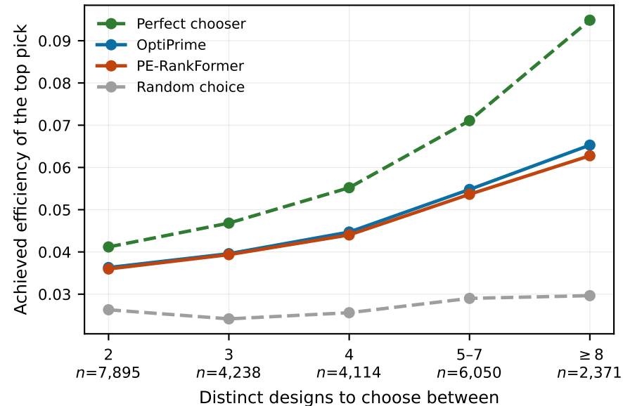
a The choice gets harder with depth
