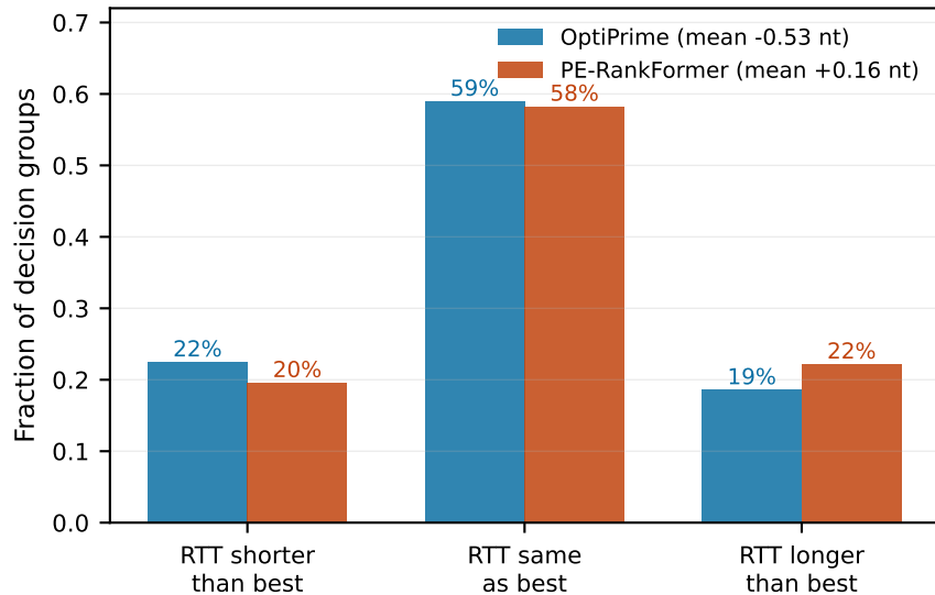
b The two models err in opposite directions
