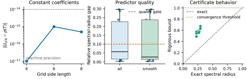
Fig. 1 Spectral validation. Left: the Fourier envelope is exact in constant-coefficient periodic systems. Middle: the four-corner predictor has a small spectral-radius gap in smooth variable-coefficient cases. Right: the signed rate certificate is rigorous but conservative.
