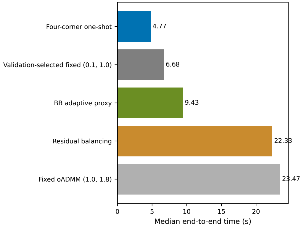
FIRE 256 runtime
