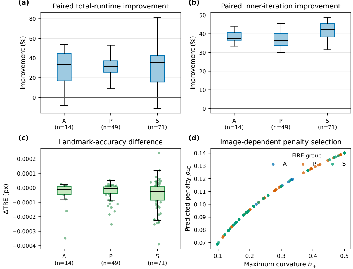
Figure 2: FIRE registration at 256 \times 256 . (a) Pairwise total-runtime reduction and (b) inner-iteration reduction relative to the validation-selected fixed comparator. (c) \Delta TRE = TRE_{4C} - TRE_{\text{fixed}} , where “fixed” denotes that comparator. (d) Predicted penalty versus image-dependent maximum data curvature.
