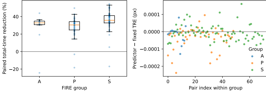
Figure 5: Complete FIRE paired comparison. Left: total-time reductions by benchmark group. Right: paired landmark-error differences; zero denotes equal median TRE. The predictor improves runtime in every group without a systematic TRE shift.
