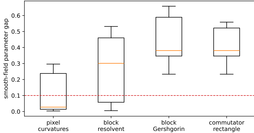
Figure 2: Smooth-field parameter gaps. The four-corner predictor (exactly equivalent here to pixelwise enumeration) passes the 0.10 empirical quality gate; rigorous structured enclosures do not.
