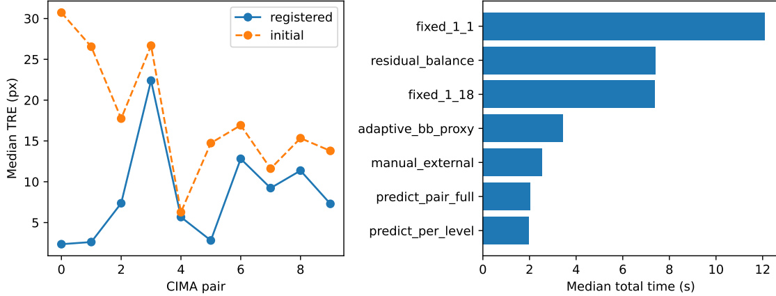
Figure 4: CIMA pairwise landmark error and matched-protocol runtime. The difficult high-TRE pair is retained rather than excluded.
