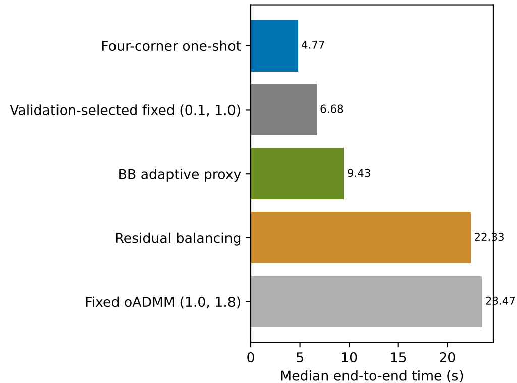
FIRE 256 runtime
