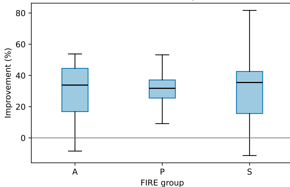
Accuracy difference
