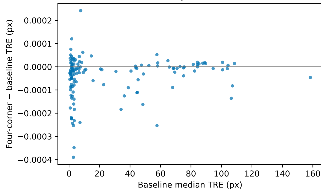
Accuracy difference
