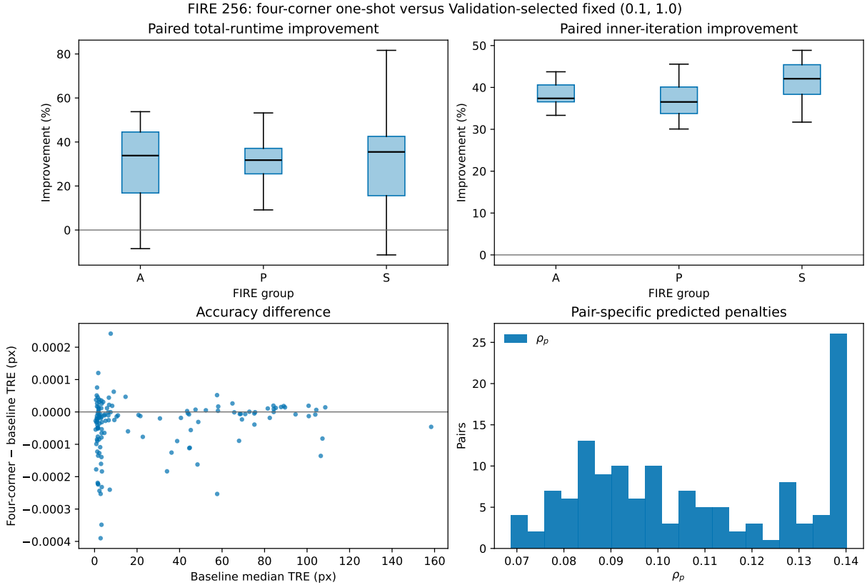
Figure 2: FIRE 256 paired analysis against the strongest practical baseline (the externally validation-selected fixed pair). Runtime and iteration improvements remain positive across groups; TRE changes are numerically negligible, and the predicted penalties vary by pair.
