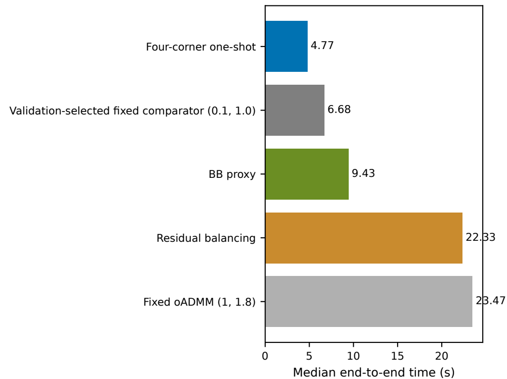
FIRE 256 runtime
