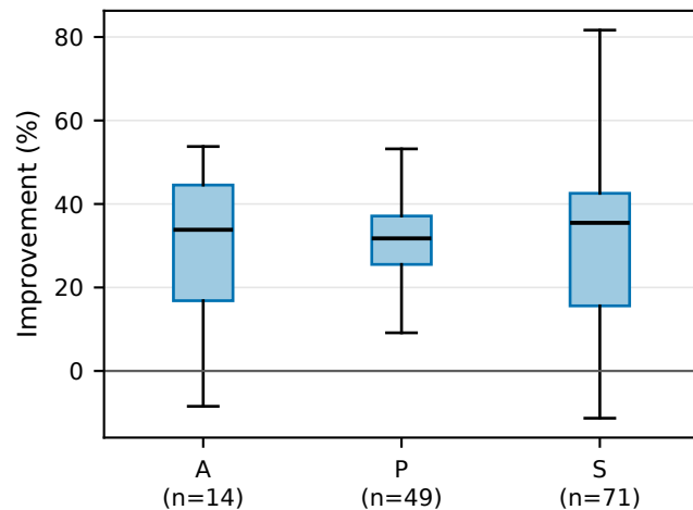
(c) Landmark-accuracy difference
