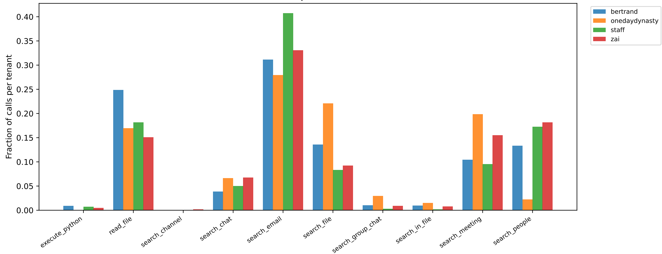
Tool Call Distribution per Tenant (Normalized)
