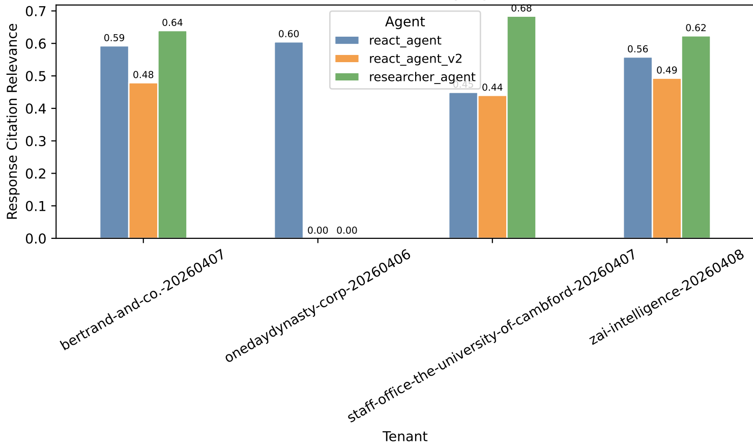
Response Citation Relevance by Agent and Tenant
