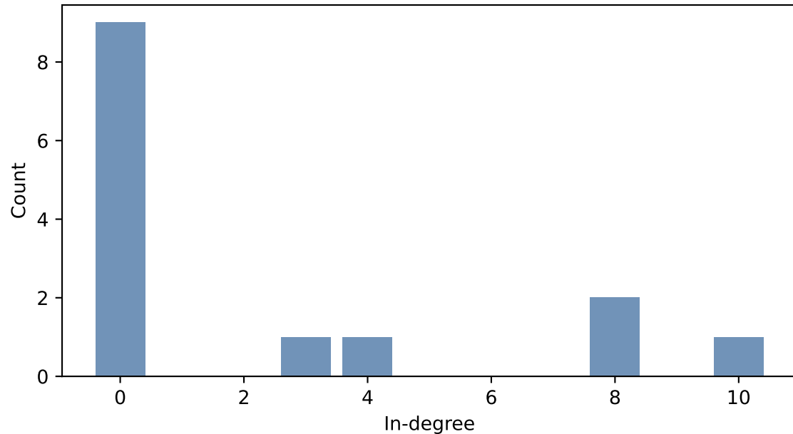
In-degree distribution
