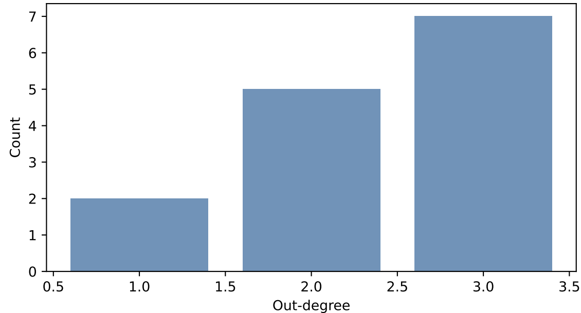
Out-degree distribution
