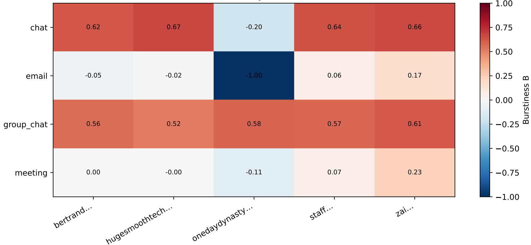
Burstiness Coefficient B per (Tenant × Channel)
