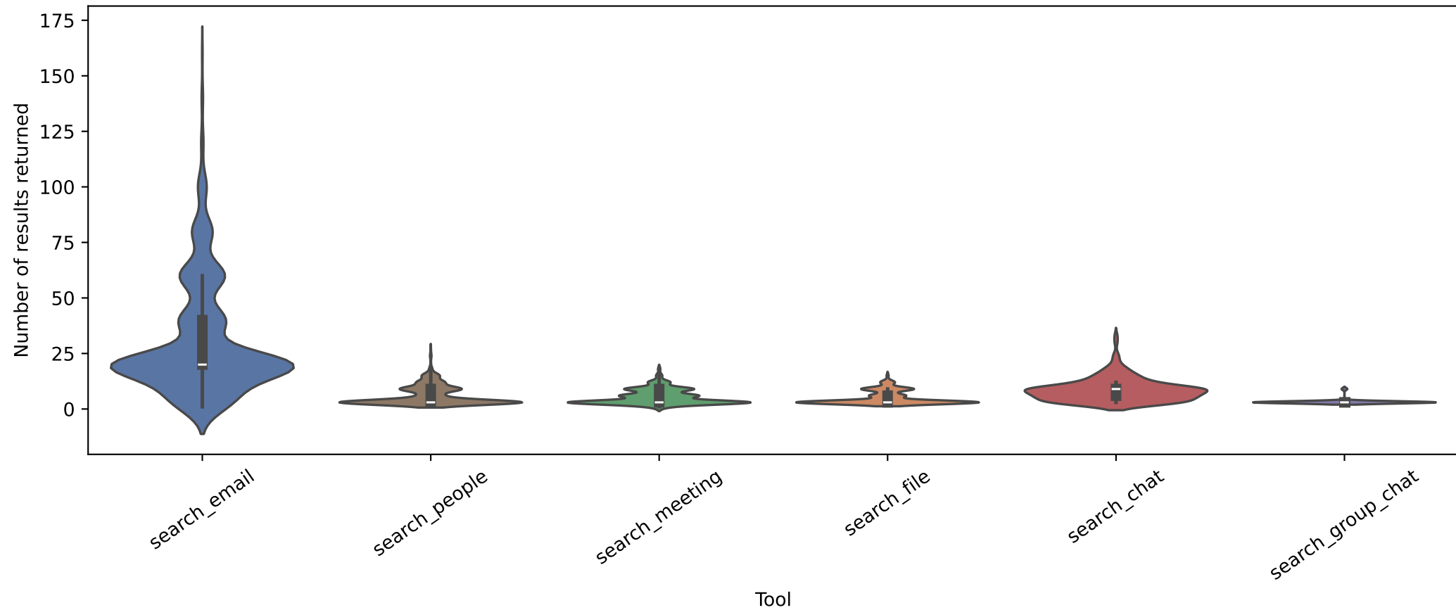
Result Count Distribution per Search Tool
