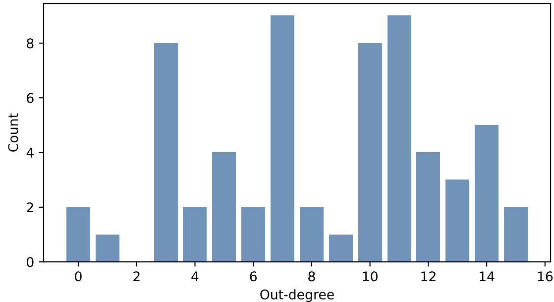
Out-degree distribution
