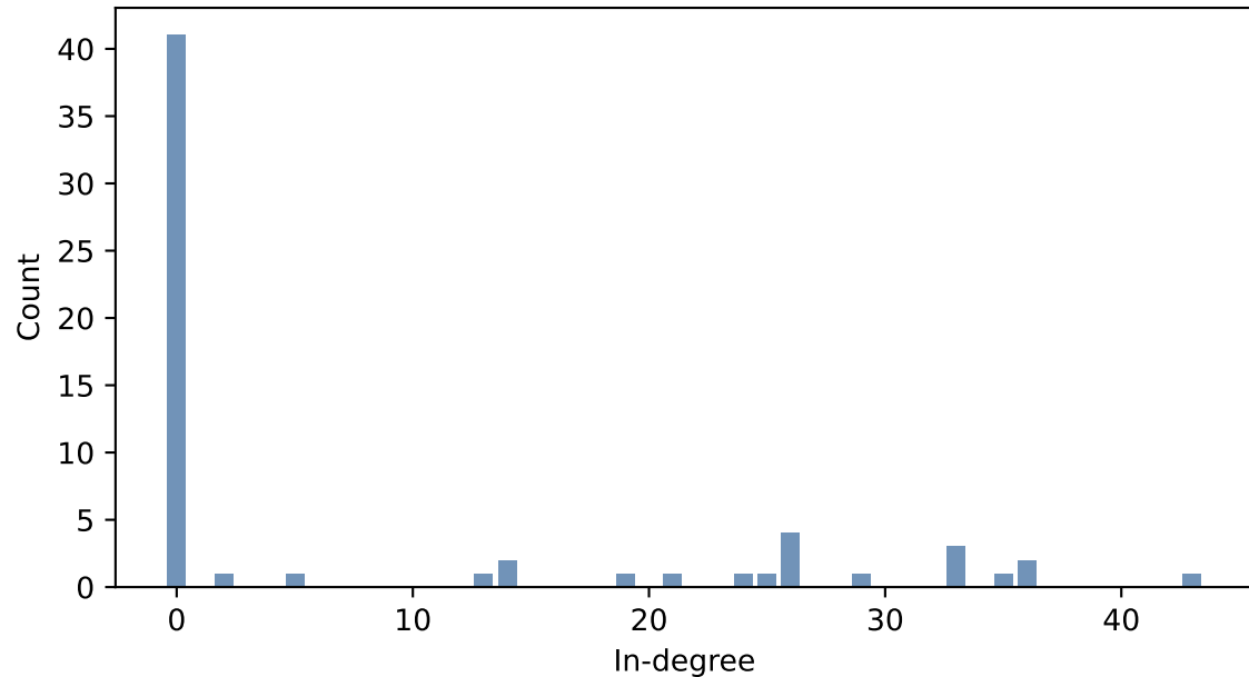
In-degree distribution
