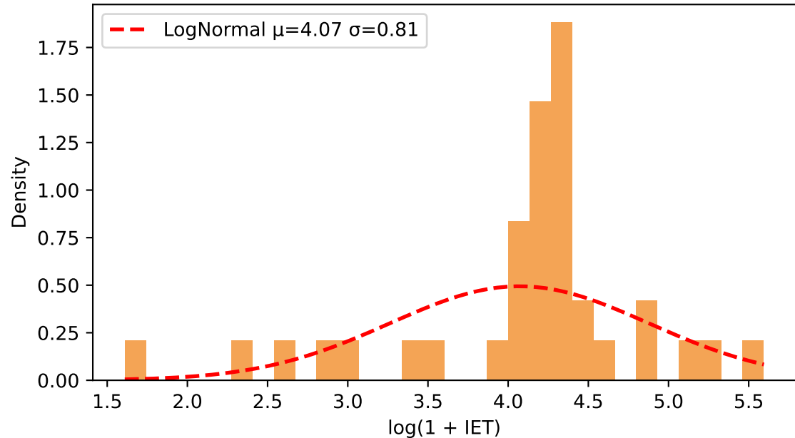
Log-scale histogram
