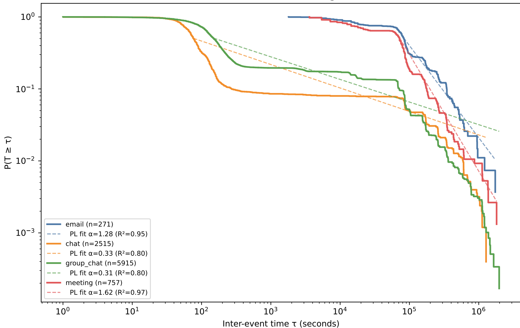
IET CCDF (all channels) — zai-intelligence-20260408
