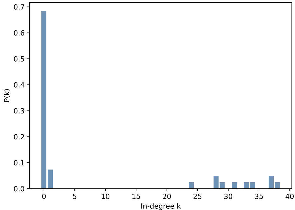
In-degree distribution (linear)
