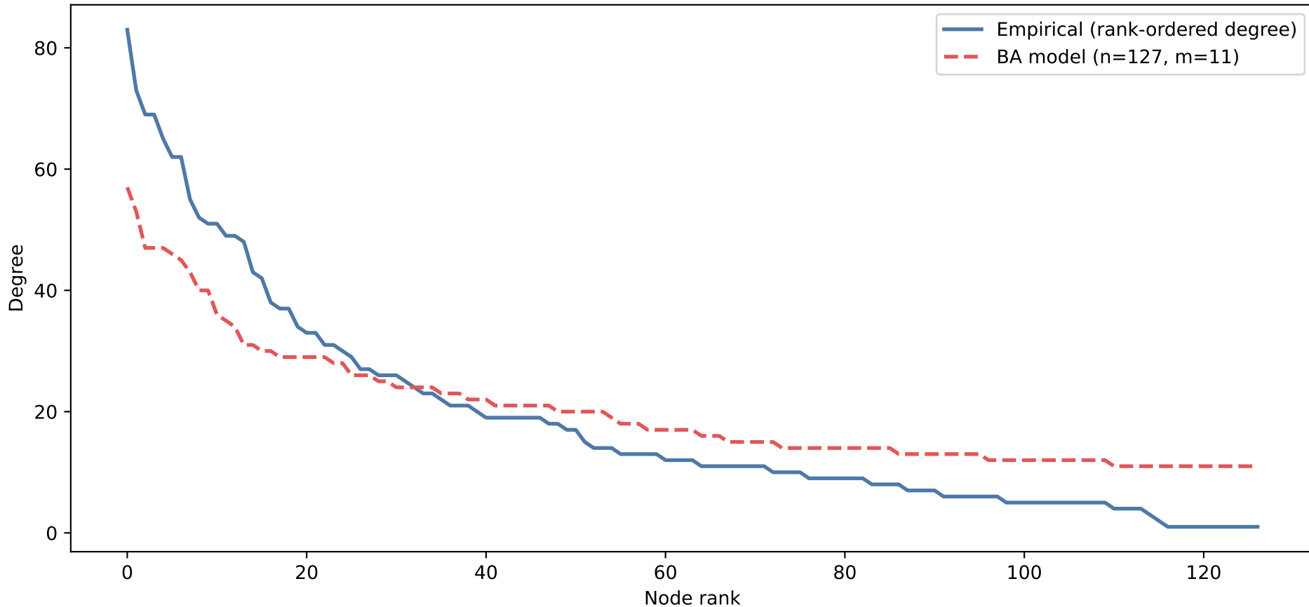
Empirical vs BA Model Degree — hugesmoothtech-corp-20260404
