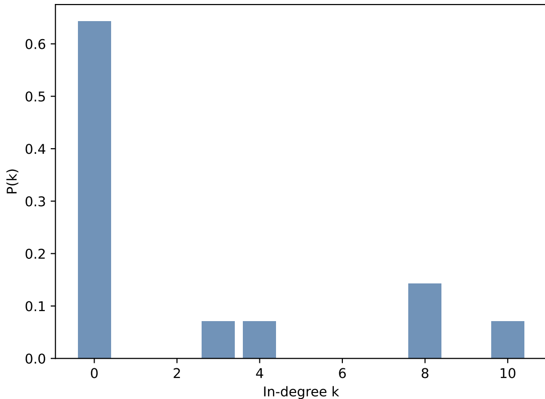
In-degree distribution (linear)
