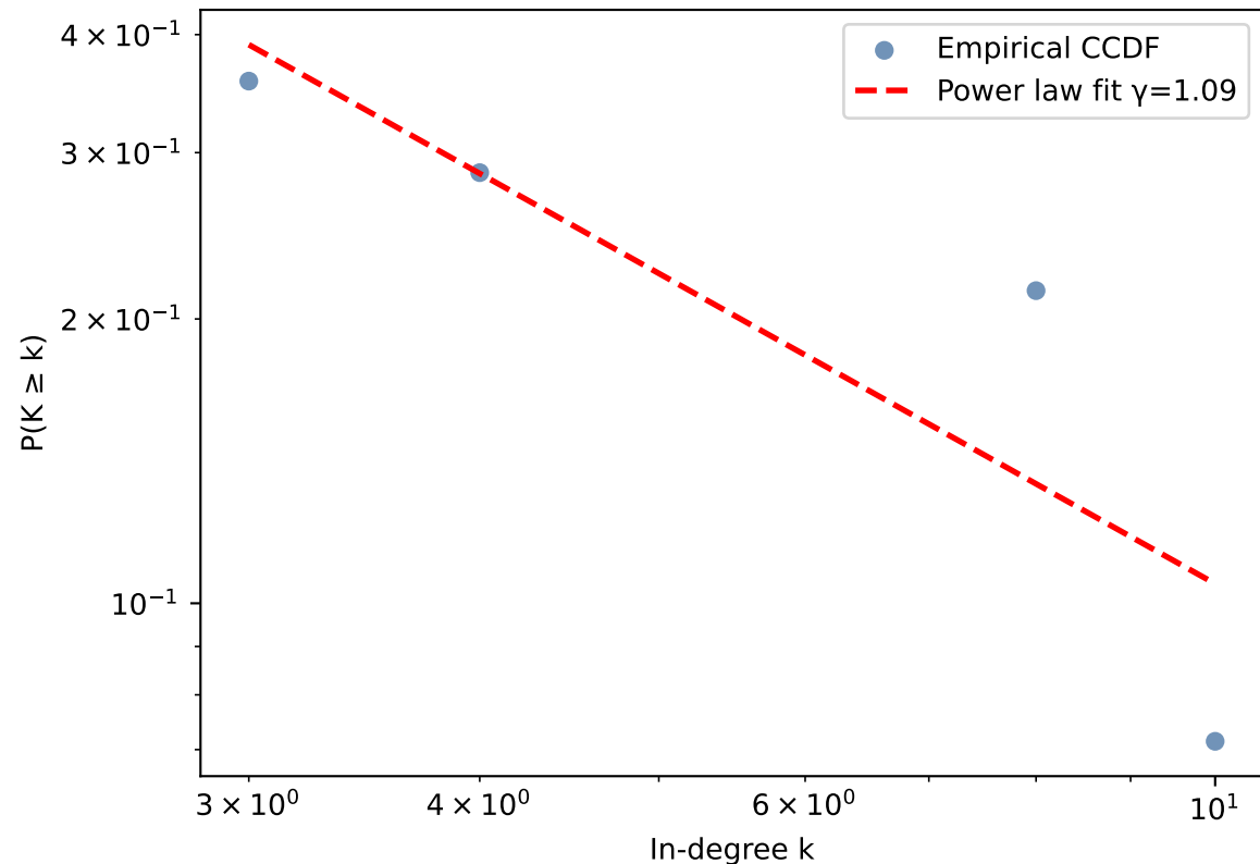
CCDF (log-log) + power-law fit
