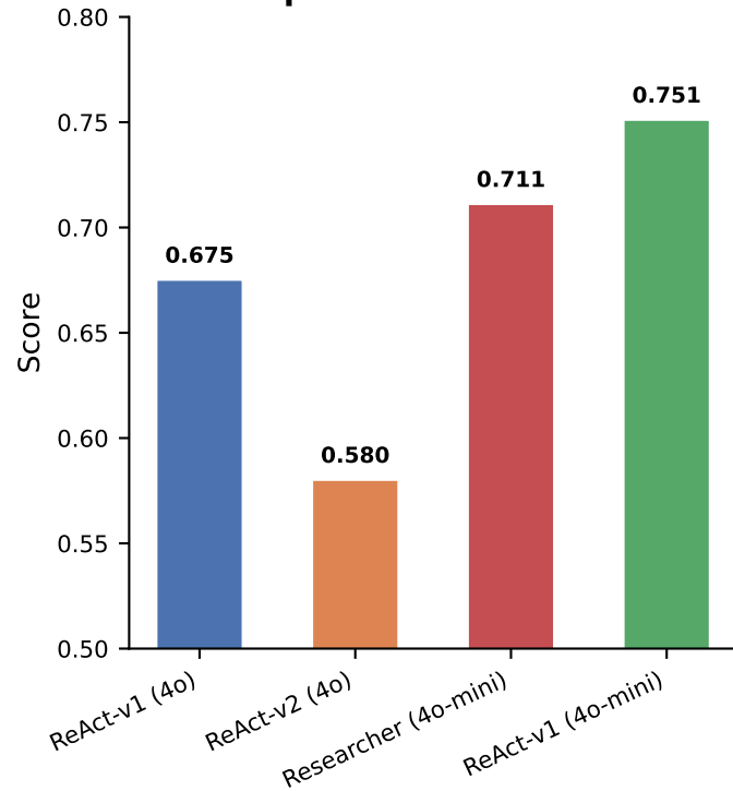
Composite Citation Score
